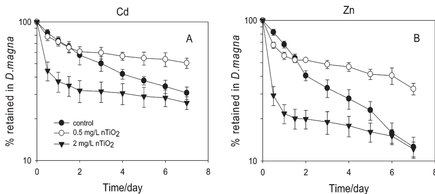
Figure 3. (A),(B) Retention of ^{109}\text{Cd} and ^{65}\text{Zn} in D. magna during 7 days of depuration in Elenedt M7 medium after 3 days of exposure to ^{109}\text{Cd} - and ^{65}\text{Zn} -radiolabeled nano-TiO 2 (0.5 and 2 mg/L). The control treatment contained only the dissolved metals. Values are mean \pm SD ( n = 3 ).
