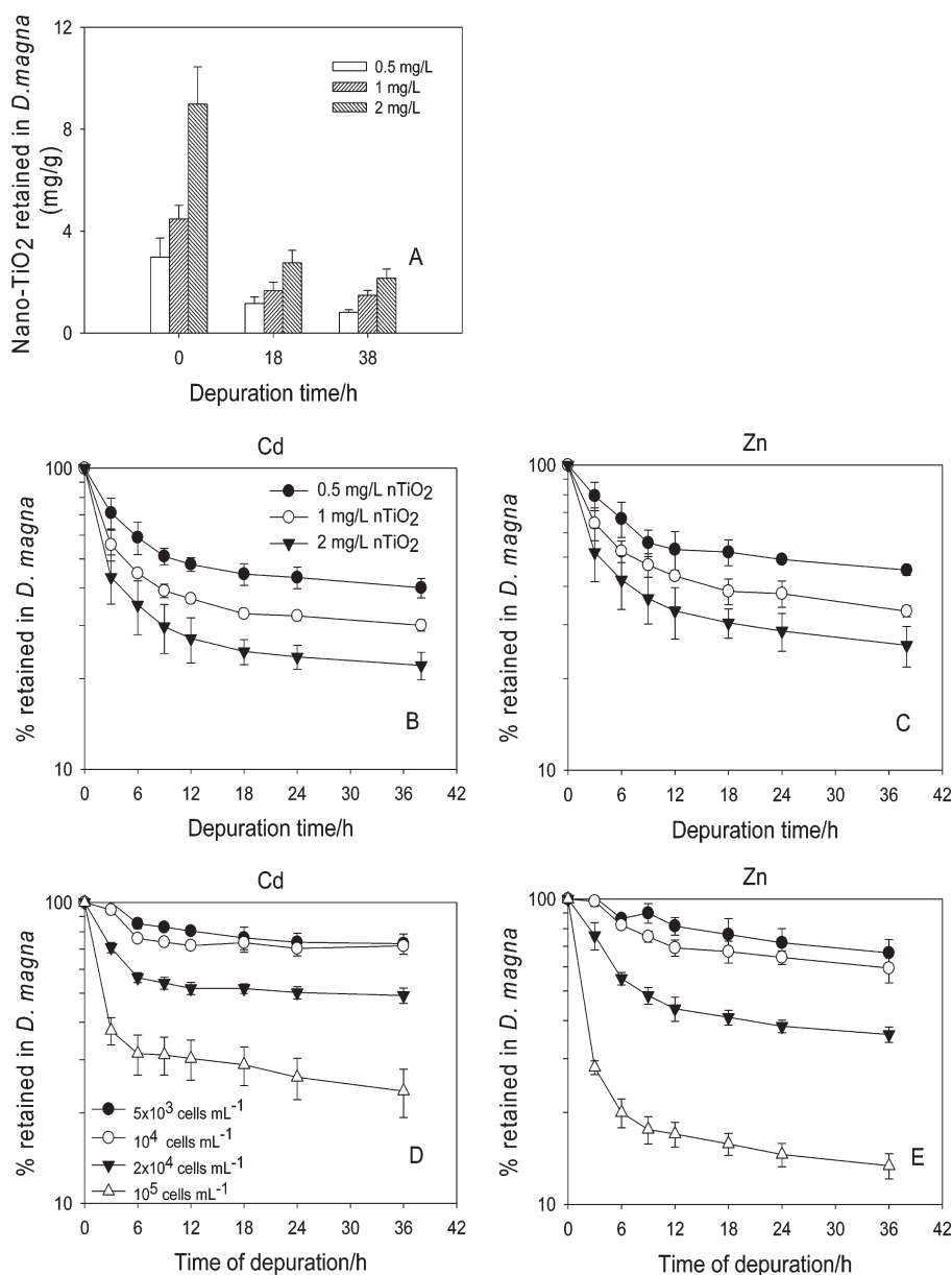
Figure 2. (A) and (B) and (C) Retention of ingested nano-TiO 2 and 109 Cd and 65 Zn in D. magna following a 15 min pulse exposure to nano-TiO 2 at different concentrations. (D) and (E) Retention of ingested 109 Cd and 65 Zn in D. magna following a 15 min pulse feeding on algae at different concentrations. The algae were spiked with 109 Cd- and 65 Zn-radiolabeled nano-TiO 2 . Values are mean ± SD ( n = 3).
